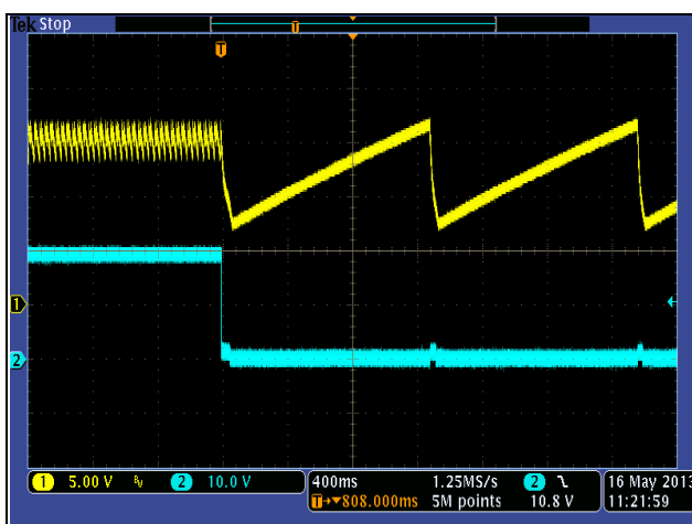
Output Short Protection Vin: 90Vac O/P : +19V=0A→Short CH1: Vcc CH2: V_{O+19V}
