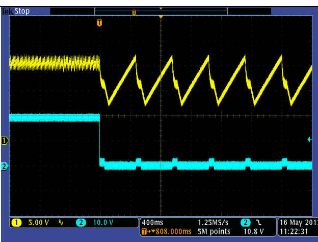
Output Short Protection Vin: 264Vac O/P : +19V=0A→Short CH1: Vcc CH2: V_{O+19V}
