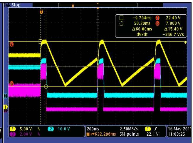
Over Voltage Protection Test
