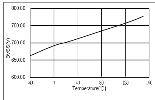
Fig. 2 LD9534 Breakdown Voltage vs. Temperature
