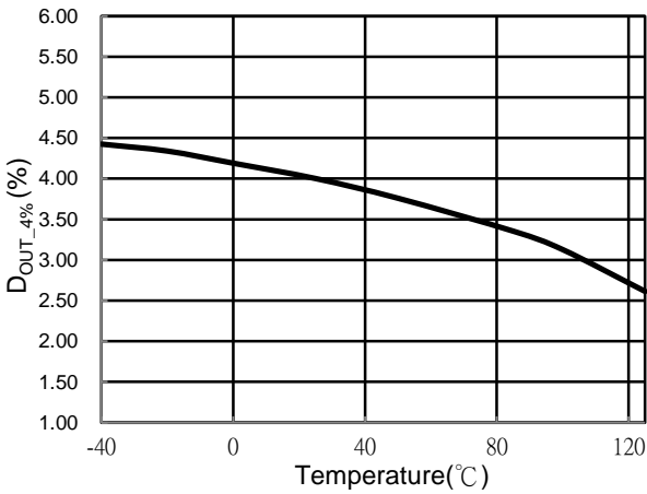
Fig.10 D_OUT_4% VS. Temperature
