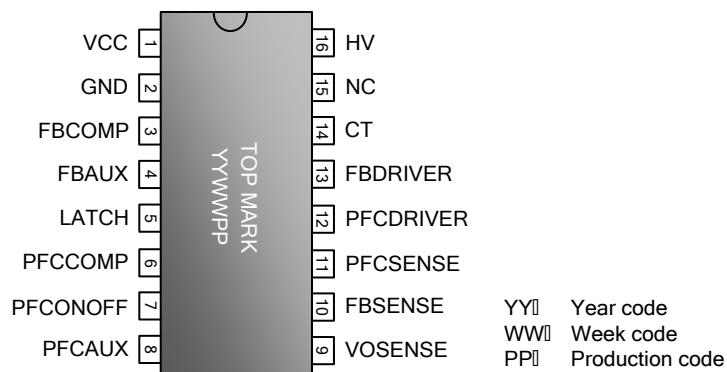
SOP-16 (TOP VIEW)
